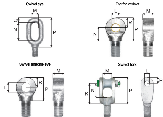
Top fittings
