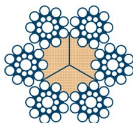
6x19 (9/9/1) Poly Core
