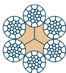
6x26* (10/5&5/5/1) Poly Core
