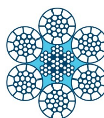
6x26 (10/5&5/5/1) IWRC
